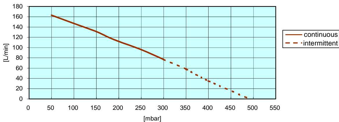
HP 120 Q-H Performance Curves
